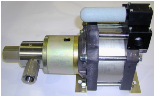
GSF15 (L) single acting, single air drive head with distance piece (Standard= Bottom inlet)
